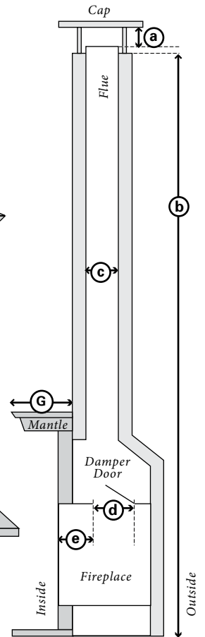
Side View
